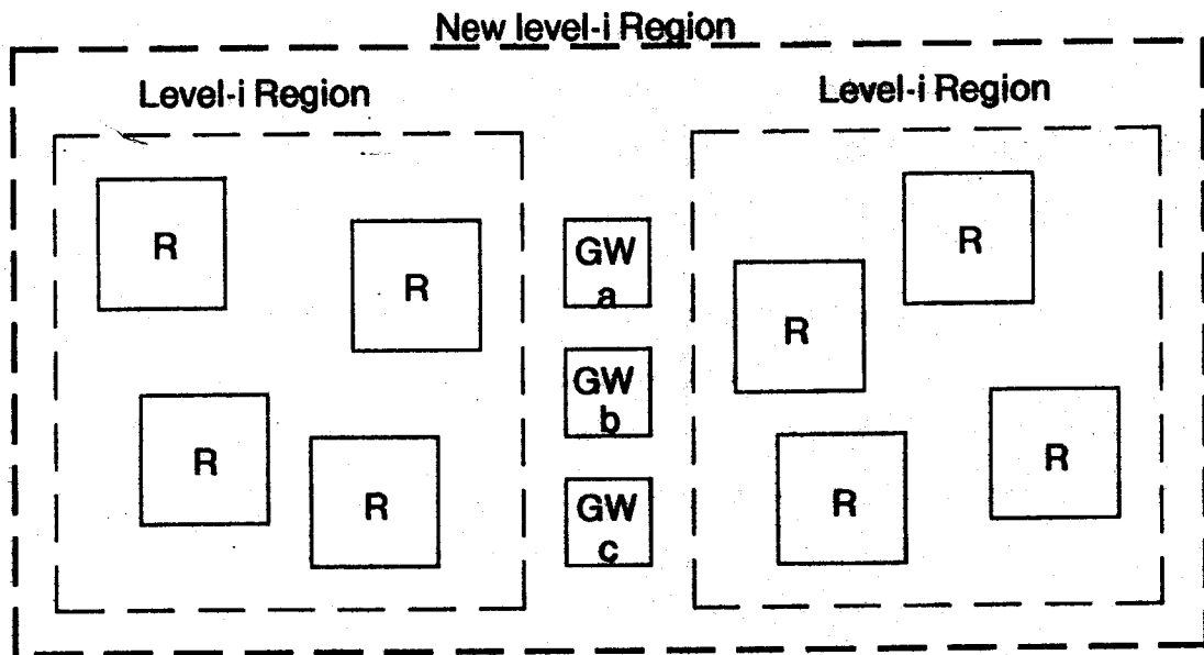
Figure 3-8: Merging two level-i regions
